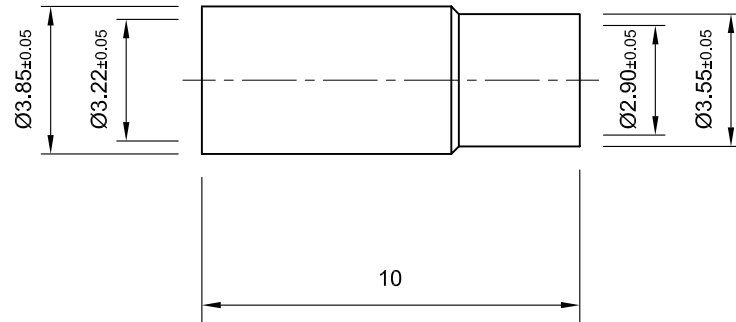
RECOMMENDED STRIPPING DIMS
